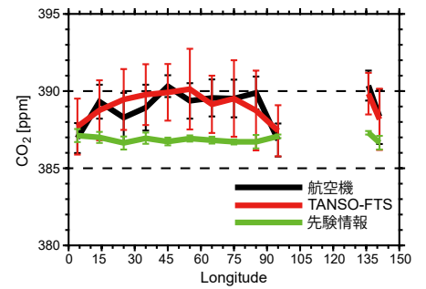
日本-ヨーロッパ間の GOSAT/TANSO-FTS と航空機の上部対流圏の二酸化炭素濃度データの比較結果（Saitoh et al. [AMT, 2016] の図 6b より改変） Comparisons of upper tropospheric CO 2 concentrations between GOSAT/TANSO-FTS and aircraft data during flights between Japan and Europe (modified from Figure 6b of Saitoh et al. [AMT, 2016])
